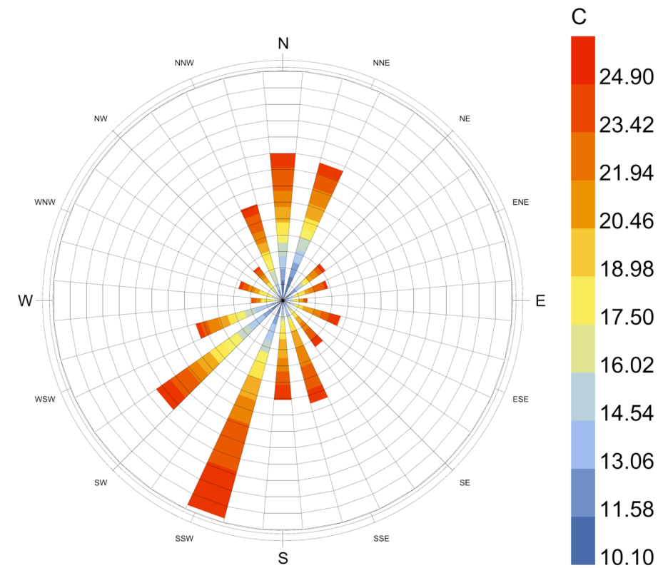
Dry Bulb Temperature (C) city: Dalian country: CHN time-zone: 8.0 source: CSWD period: 1/1 to 12/31 between 0 and 23 @1
