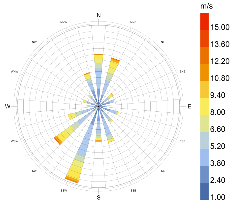
Wind Speed (m/s) city: Dalian country: CHN time-zone: 8.0 source: CSWD period: 1/1 to 12/31 between 0 and 23 @1
