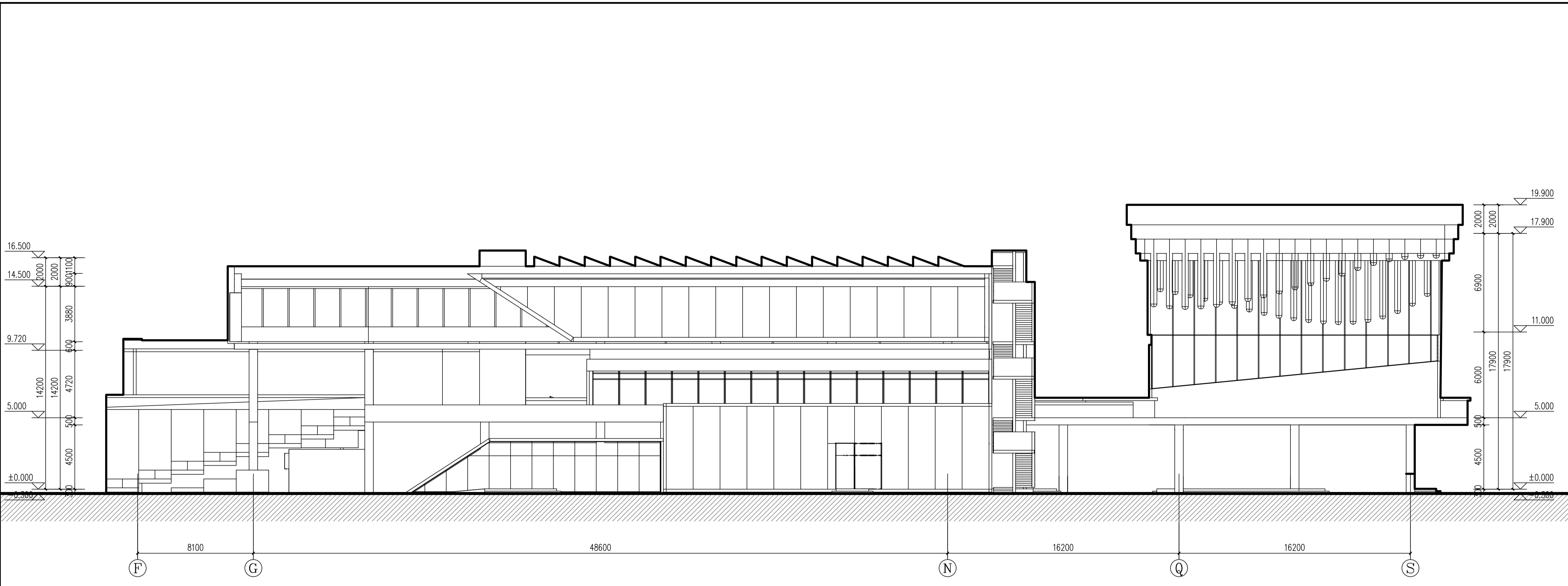
F-S轴立面图:150
